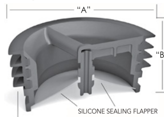
SILICONE GASKET FLEXES .100" TO FIT DIAMETER
